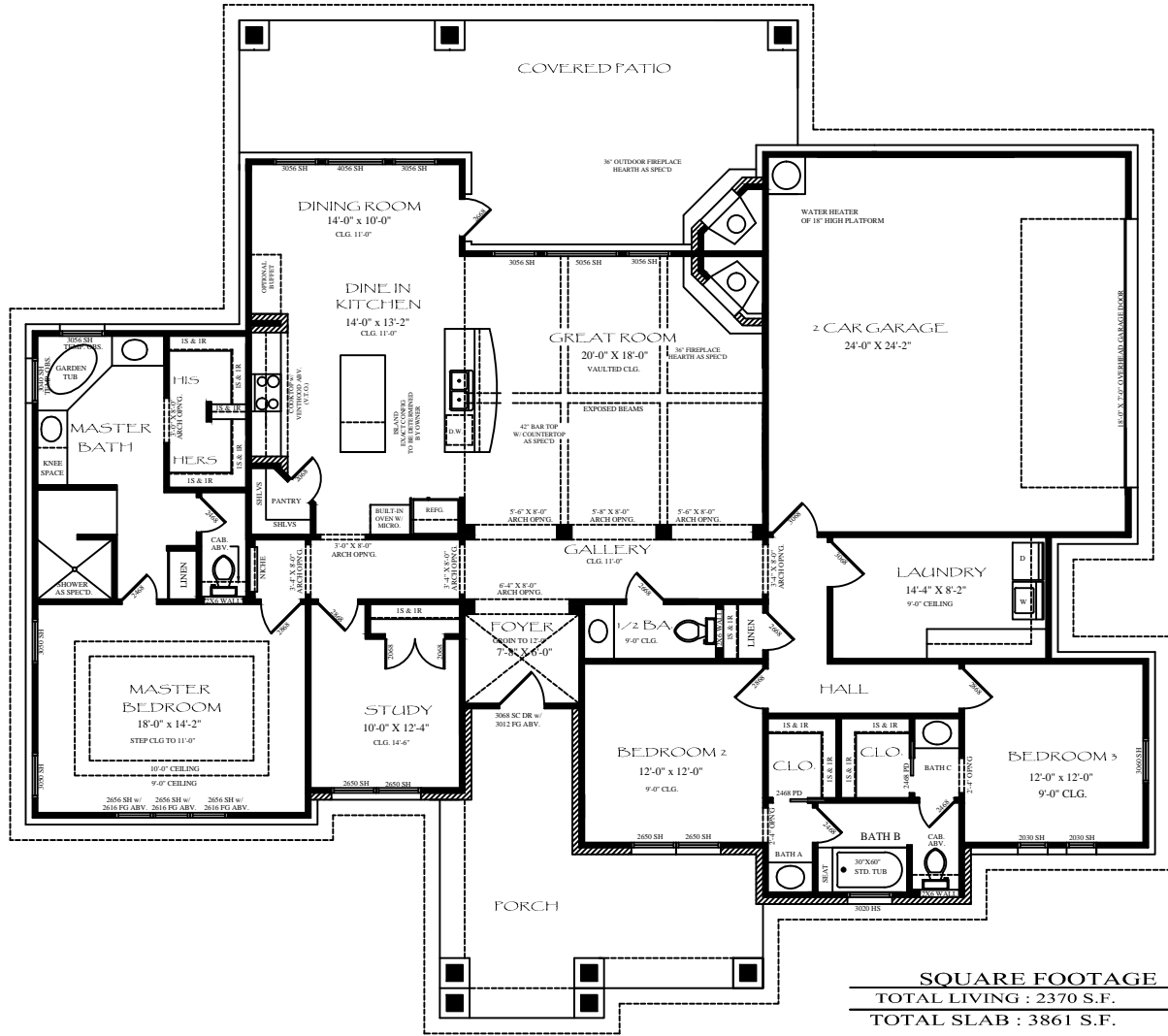
FLOOR PLAN
