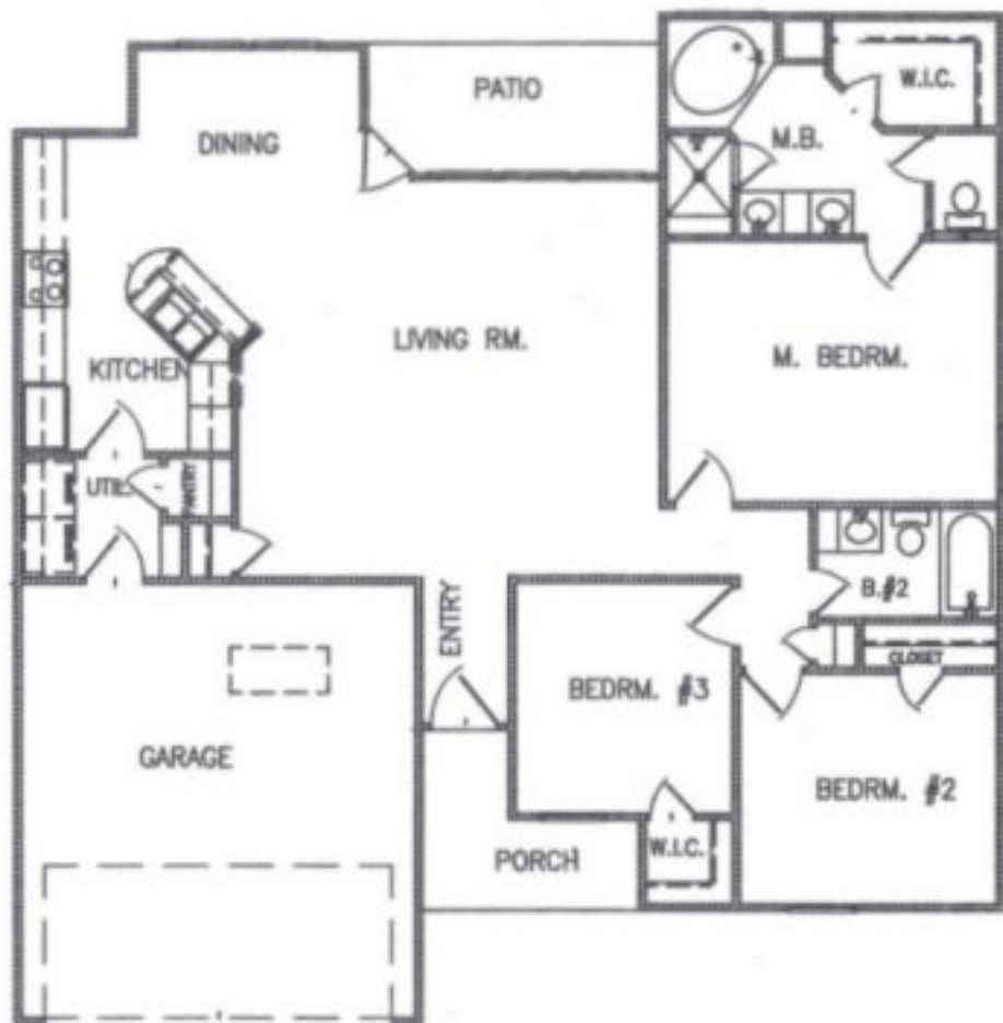
RANCH COUNTRY COUSTOM HOMES FLOOR PLAN MODEL- 1397
