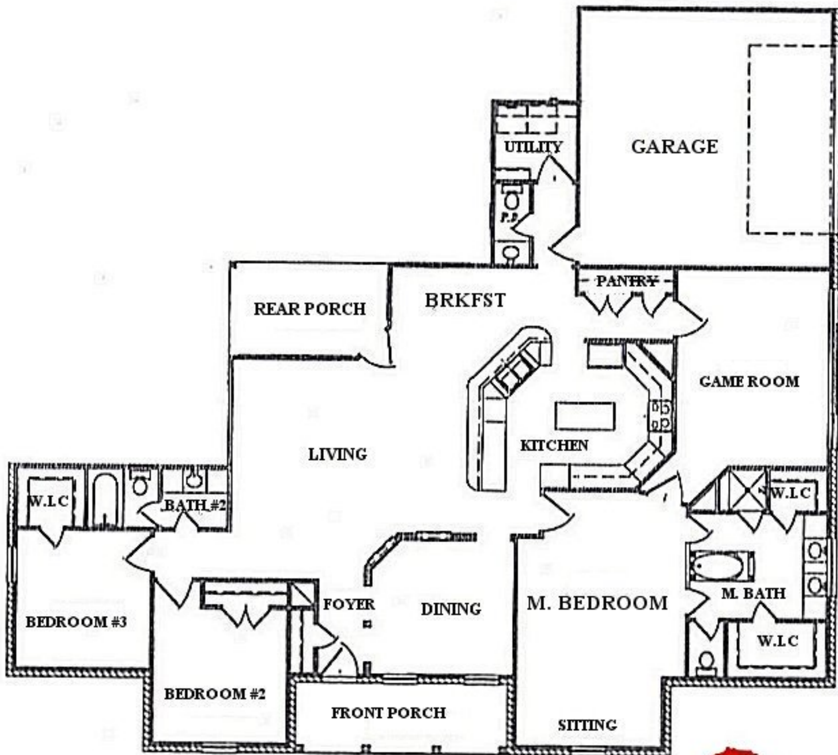
RANCH COUNTRY CUSTOM HOMES PLAN DWG. DENVER III 2,235 SQ. FT. LIVING FLOOR PLAN
